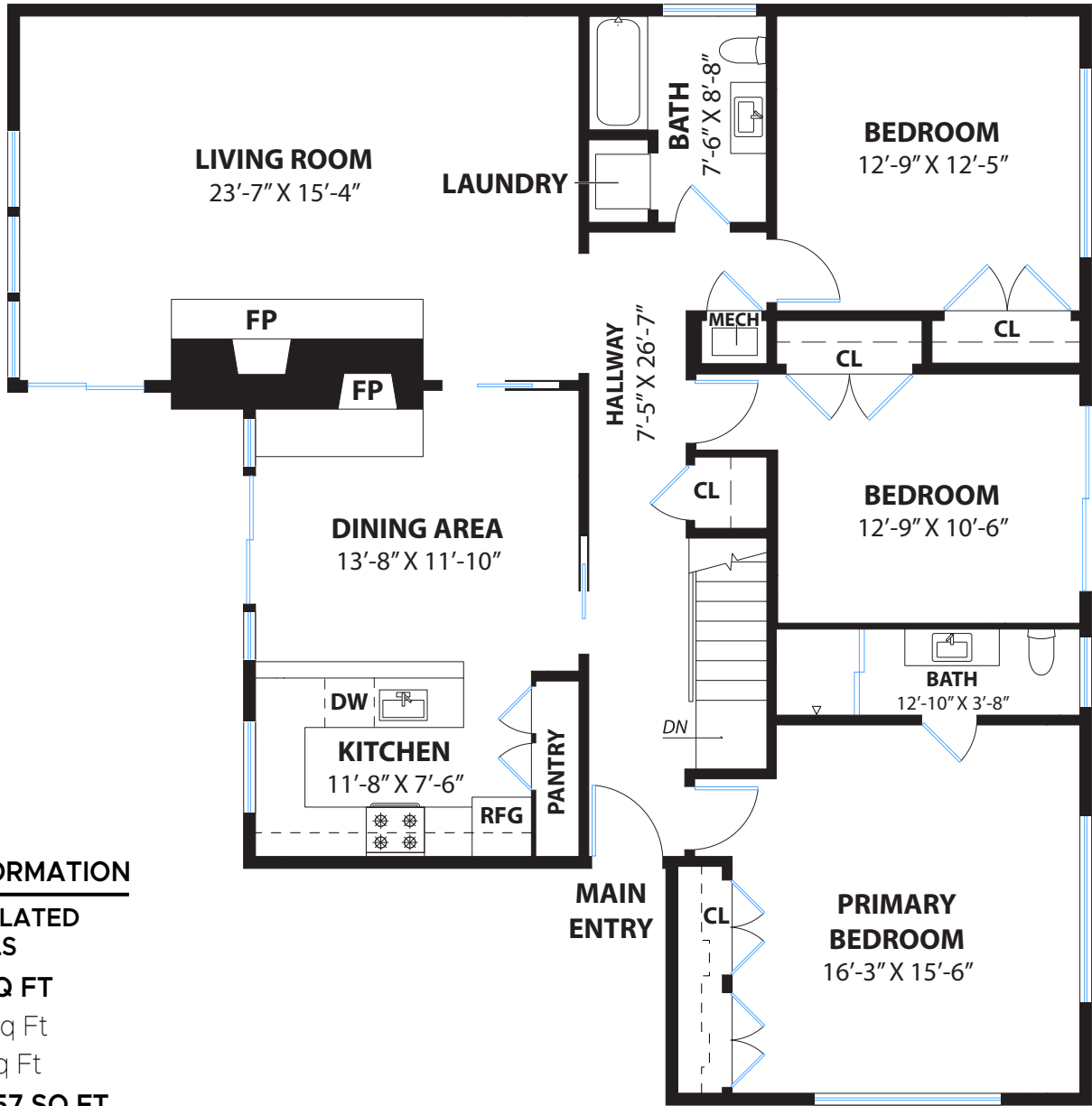
MAIN LEVEL
